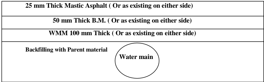
H) Cross Section for Reinstatement of Trenches in UTWT Road
