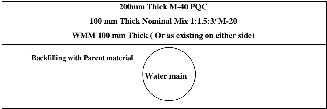
F) Cross Section for Reinstatement of Trenches in Footpath M-20
