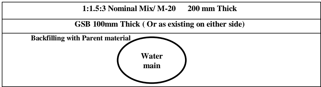
G) Cross Section for Reinstatement of Trenches in Mastic Asphalt
