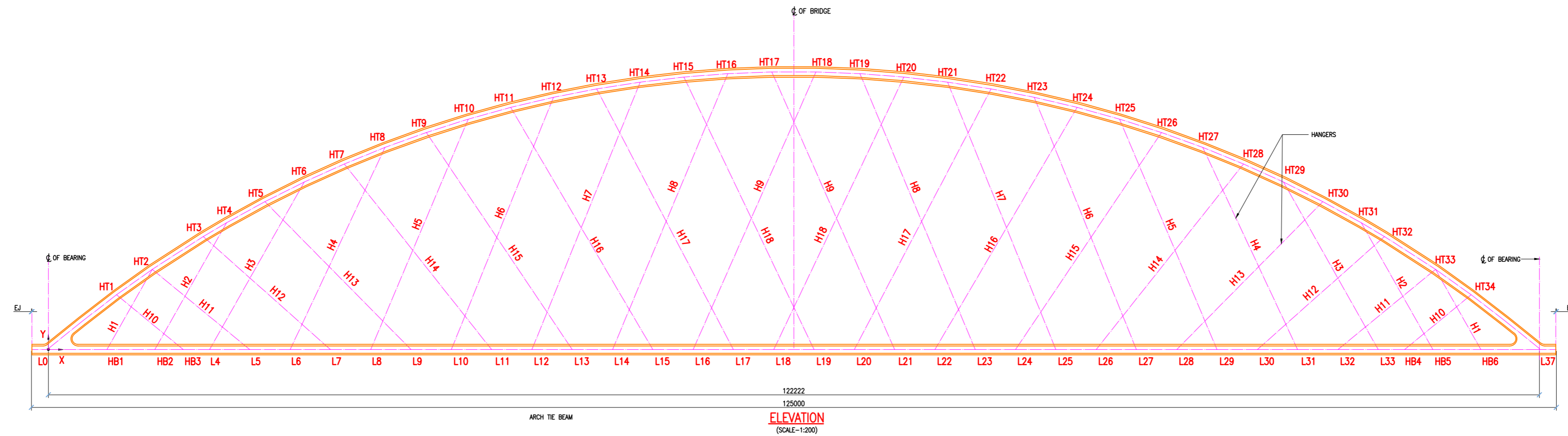
SHOWING TYPICAL ARRANGEMENT OF HANGERS FOR NETWORK ARCH
