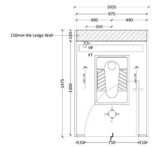
PLAN INDIAN WC CUBICLES
