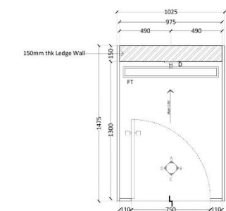
PLAN SHOWER CUBICLES
