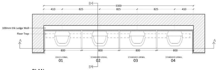
PLAN MALE URINAL AREA
